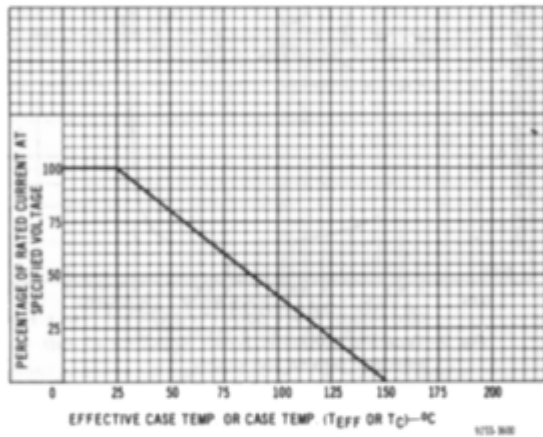
Fig. 1 - Derating curve for all types.
