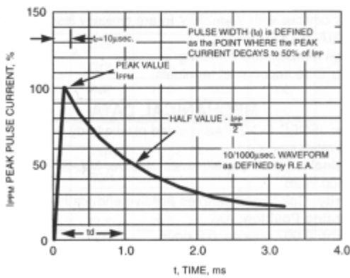
FIG. 3 - PULSE WAVEFORM
